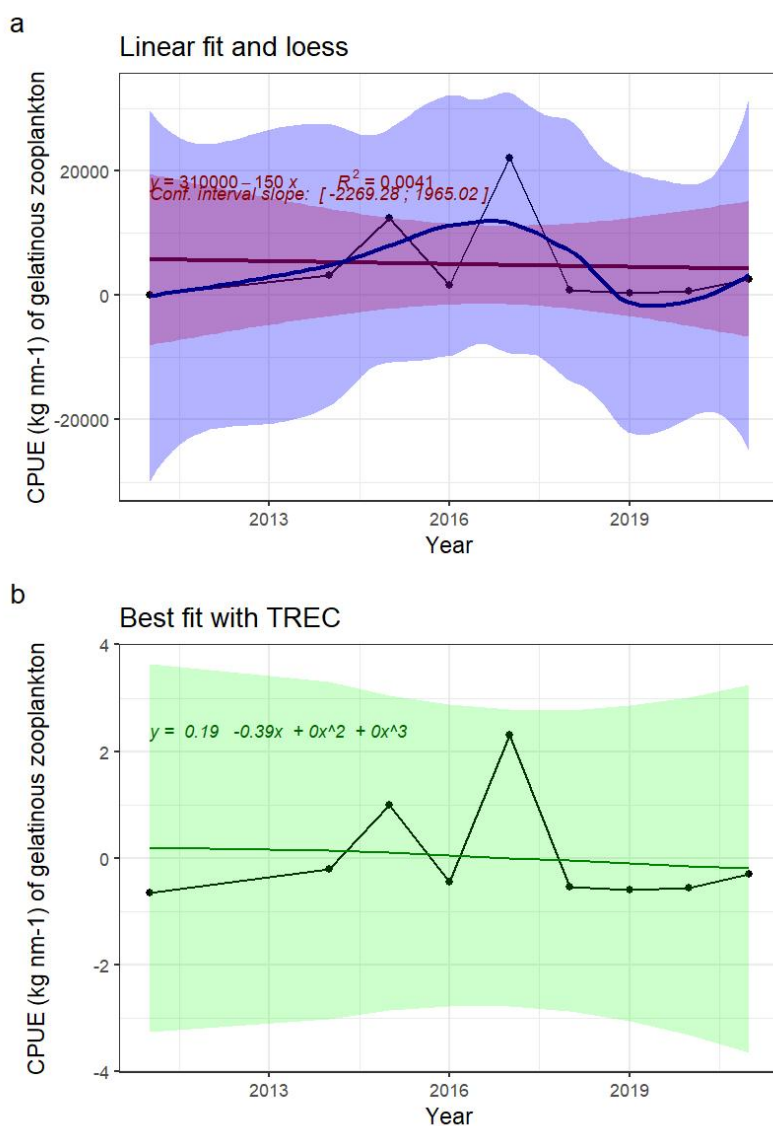
Figure 10: Indicator time series and fitted trends. A) linear trend fitted with Least-square method (not adapted for short time series) in red, and loess in blue, for information. B) Best fitted trend using the first steps of a TREC analysis on standardized time series
