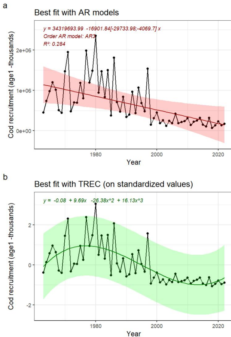
Figure 16: A) Indicator time series and best fitted trend with autoregressive model (AR0: no autoregression; AR1: 1 st order autoregressive model, AR2: 2 nd order autoregressive model, AR3: 3 rd order autoregressive model). Numbers in brackets indicate the confidence interval (95%) around the slope coefficient and should not include 0 to be significant. B) Best fitted trend using the first steps of a TREC analysis on standardized time series
