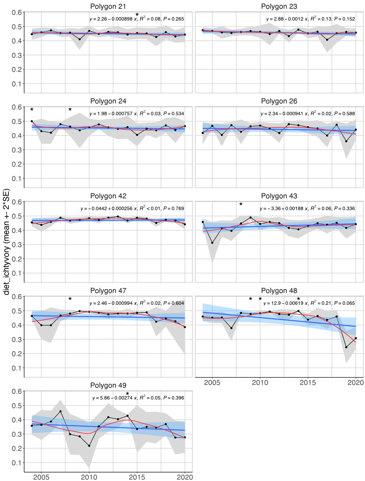
Figure A.3.7. Mean ( \pm 2*SE ) biomass proportion of the ichthyivorous feeding guilds in the Arctic Barents Sea (Black dots and grey shading). Linear regression fit with 95% CI is shown in blue, and the statistical results are given in the top of each plot. A local smoother is added in red to assist visual interpretation of non-linear changes during the period. Stars indicate years with low sample size (< 5 trawls).
