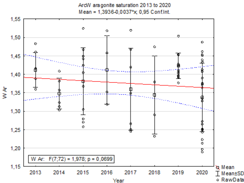
Figure A.42.1 The time series of aragonite saturation ( \Omega_{\text{Ar}} = \text{WAr} ) in the period 2013 to 2020 in the Arctic core waters ( T < 0^\circ \text{C} , > 40 \text{ m} ). The linear fit (red line) is based on annual mean values (black squares) from observational data (circles). The blue hashed lines denote the area of 95% confidence.
