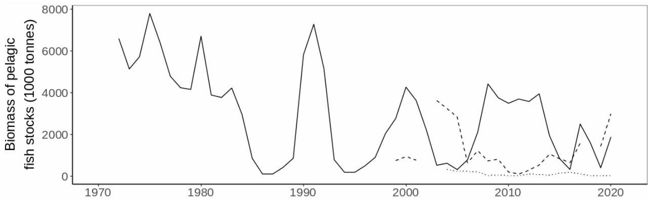
Figure A.7.1 Total annual stock biomass of capelin (solid line), herring (stippled line, missing data from 2002 and 2018) and blue whiting (dotted line).
