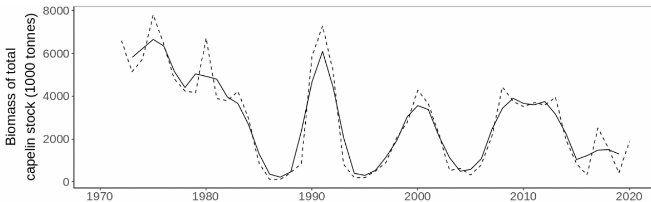
Figure S.22.2 Comparison of annual total stock estimates (stippled line) and three-year running average (solid line).
