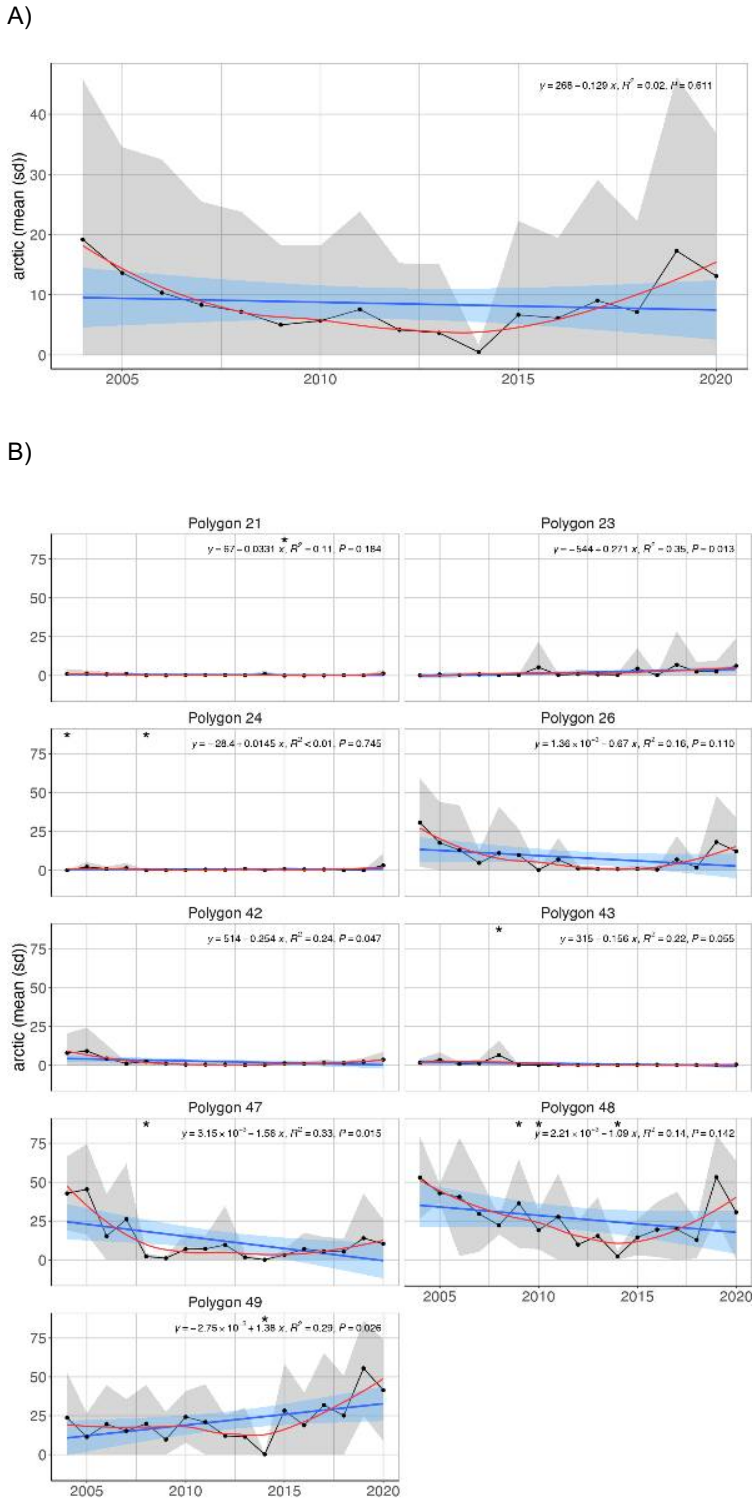
Figure A.31.2 Mean ( \pm sd) percentage based on abundances of Arctic fish species in demersal trawls the Arctic Barents Sea (Black dots and grey shading). Linear regression fit with 95% CI is shown in blue, and the statistical results are given in the top of each plot. A local smoother is added in red to assist visual interpretation of non-linear changes during the period. Stars denote years with low sample size (< 5 trawls). A) in the whole area. B) per polygons.
