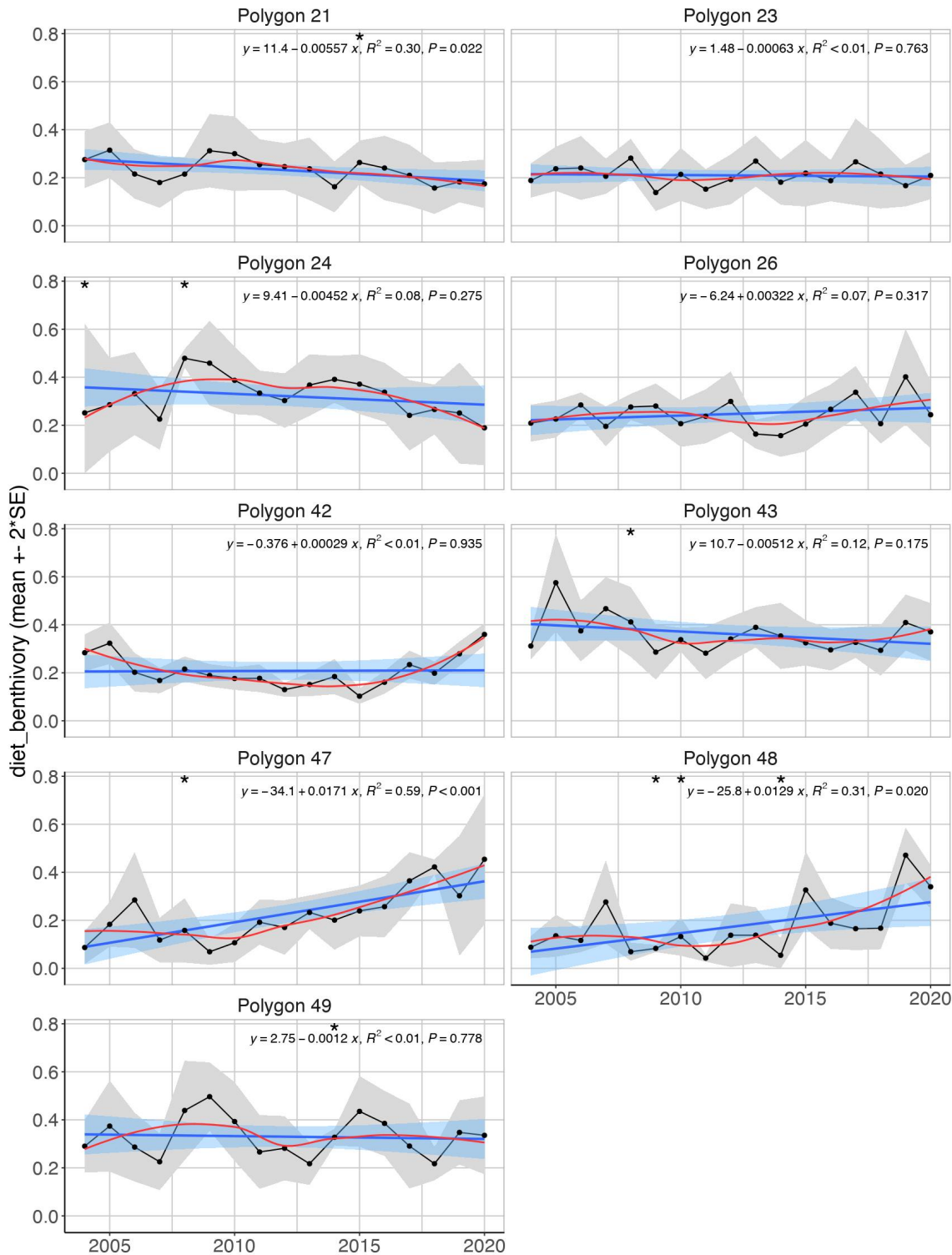
Figure A.3.6. Mean ( \pm 2*SE ) biomass proportion of the benthivorous feeding guilds in the Arctic Barents Sea (Black dots and grey shading). Linear regression fit with 95% CI is shown in blue, and the statistical results are given in the top of each plot. A local smoother is added in red to assist visual interpretation of non-linear changes during the period. Stars indicate years with low sample size (< 5 trawls).
