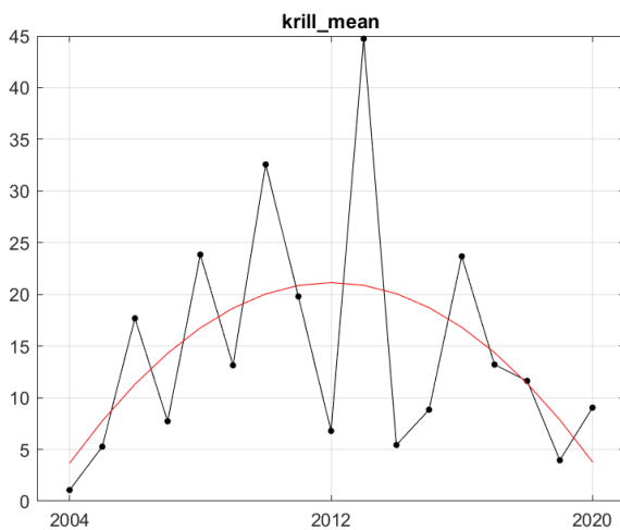
Figure S. 21.2. Estimated biomass of krill (kg wet wt. km 2 ) and fitted trend using the best fitted trend approach represented by the red line the red line. The fitted trend approach trend is of degree 2 (quadratic) with R^2=0.27 . Residual variation after fitting was 94.66.
