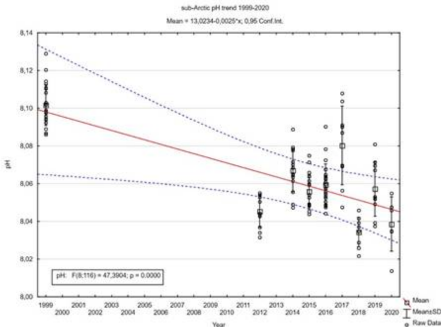
Figure S.35.1 The time series of pH in the period 1999 to 2020 in the sub-Arctic ( T > 3^\circ\text{C} ) waters. The linear fit (red line) is based on annual mean pH values (black squares) from observational data (circles). The blue dashed lines denote the area of 95% confidence.
