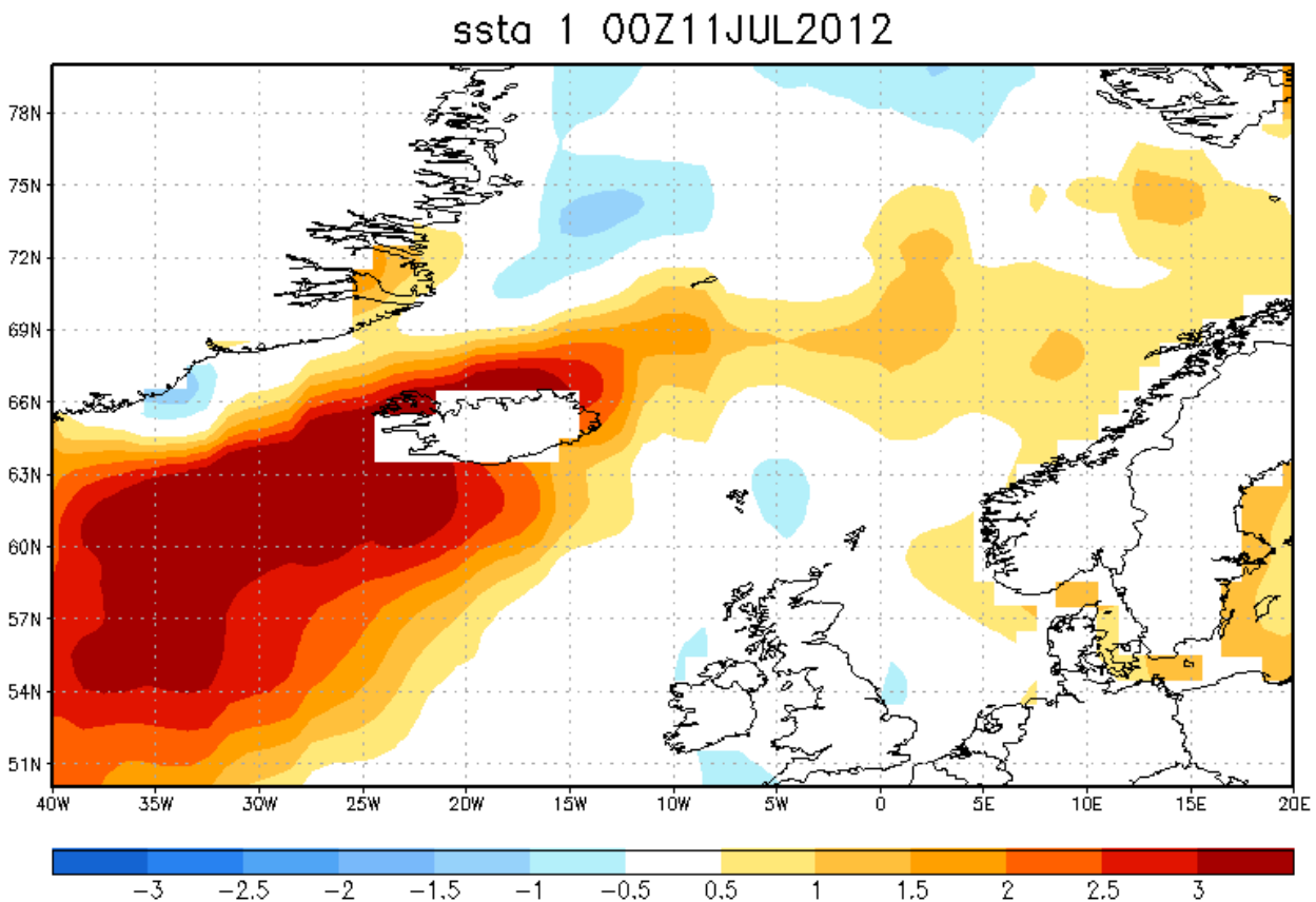
Figure 3. Sea surface temperature anomalies (°C; centered in week 28, mid July 2012) showing warm and cold conditions in comparison to a 20 year average.
