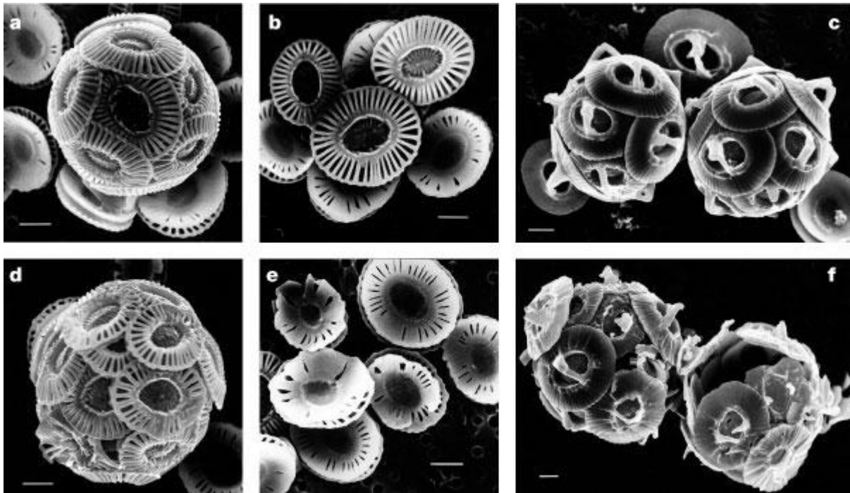
a, b, d, e, Emiliana huxleyi ; and c, f, Gephyrocapsa oceanica collected from cultures incubated at [CO 2 ] ≈ 12 μmol l -1 ( a– c ) and at [CO 2 ] ≈ 30–33 μmol l -1 ( d–f ), corresponding to pCO 2 levels of about 300 p.p.m.v. and 780–850 p.p.m.v., respectively. Scale bars represent 1 μm. Note the difference in the coccolith structure (including distinct malformations) and in the degree of calcification of cells grown at normal and elevated CO 2 levels. Pictures are selected from a large set of SEM photographs to depict the general trend in coccolith calcification. As the culture medium was super-saturated with respect to calcium carbonate under all experimental conditions, post-formation calcite dissolution is not expected to have occurred.
