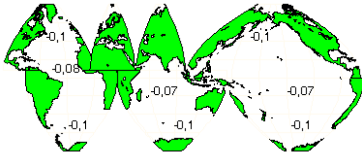
Change in pH from 1820 to 2005
